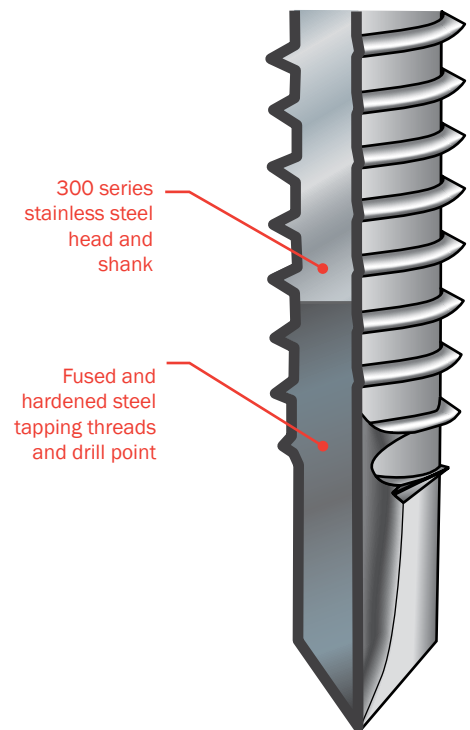
Bi-Metal Technology
