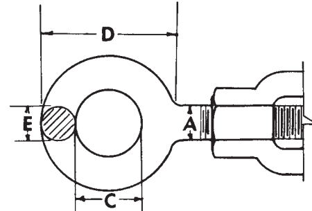
Eye DIMENSIONS – STRENGTH
