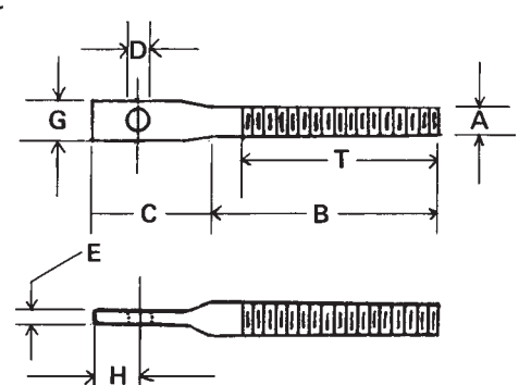
Spade Bolt
