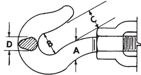
Hook DIMENSIONS – STRENGTH
